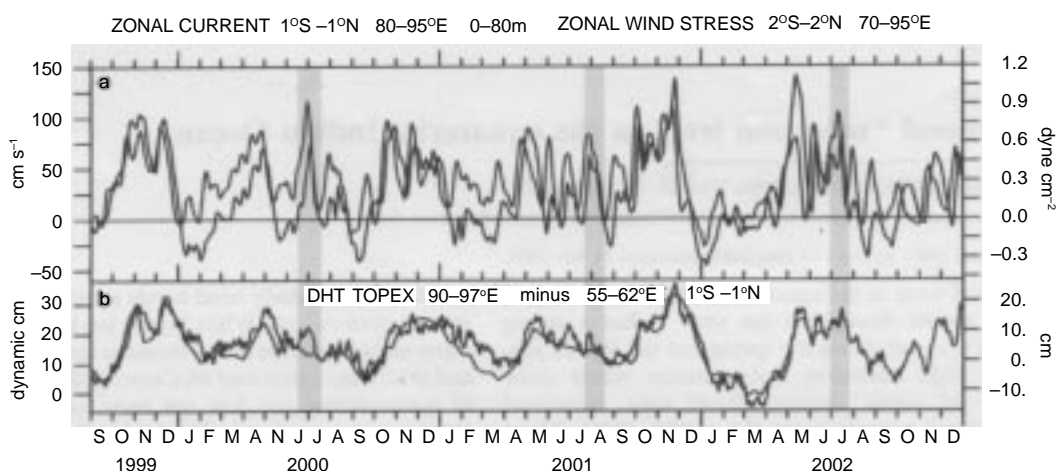
Figure 2. Time series of (a) 10-day running mean zonal wind stress (dynes cm -2 ; thin) and model daily upper ocean zonal current (cm s -1 ; bold). (b) 10-day TOPEX sea surface height anomaly (cm; thin) and model daily dynamic height (DHT; dynamic cm; bold) difference between eastern and western EqIO.
