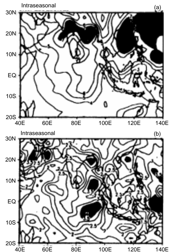
Figure 1. Geographical distribution of intra-seasonal and inter-annual activity.
