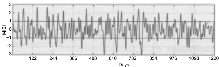
Figure 3. (a) Normalized Monsoon Intra-seasonal Oscillation Index (MISI) [29] for 10 years (each year has 122 days starting from 1954). Thin solid line corresponds to ± 1 normalized unit.
