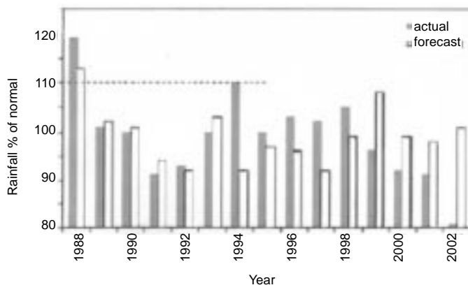
Figure 6. The performance of operational forecasts [128] between 1988 and 2002 (source : IMD, New Delhi)
